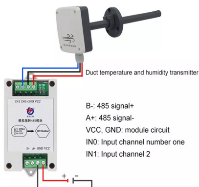
Module and three-wire transmitter connection diagram
