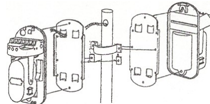
Back-to-back pole mounting.
